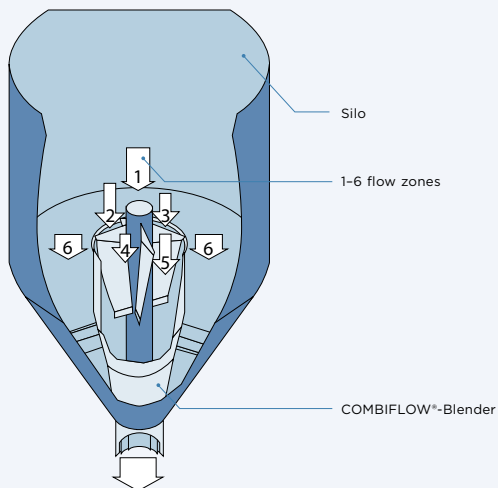
Silo cone blender CFB
