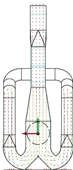
LAMINAR AIR FLOW THROUGH THE TWIN INLET DESIGN (Coperion Solution)
