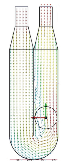
NON-LAMINAR AIR FLOW THROUGH SINGLE INLET DESIGN LEADS TO CLUMPING
