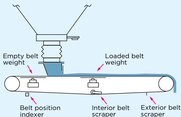
Continuous Automatic Online Belt Taring
