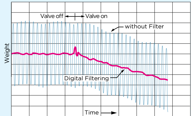
Dynamic weighing response with digital filtering vs. non-digital filtering
