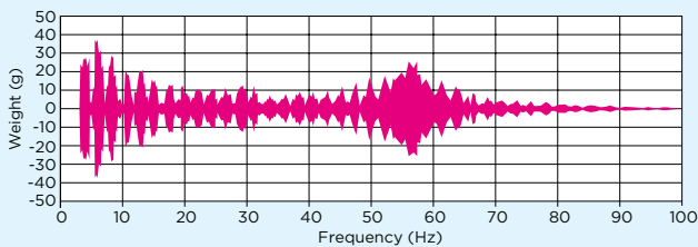
Vibrating wire sensor with digital filtering
