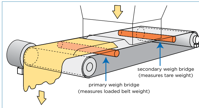
Coperion K-Tron Smart Weigh Belt feeders offer an optional secondary weigh bridge
