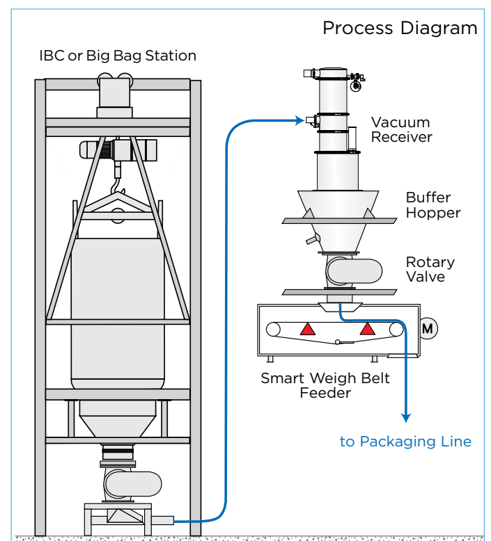
Smart Weigh Belt feeder shown with vacuum receiver, buffer hopper and rotary pre-feeder.
