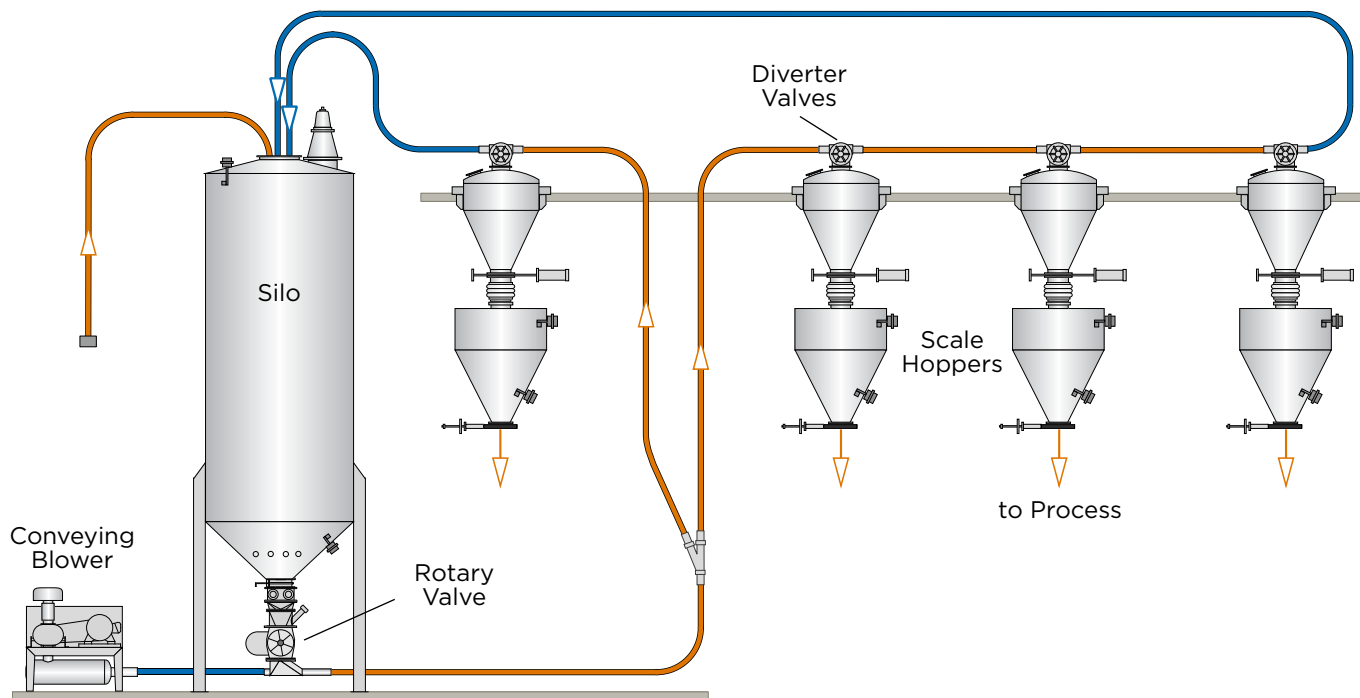
Scaling System for Multi Destination Batching
