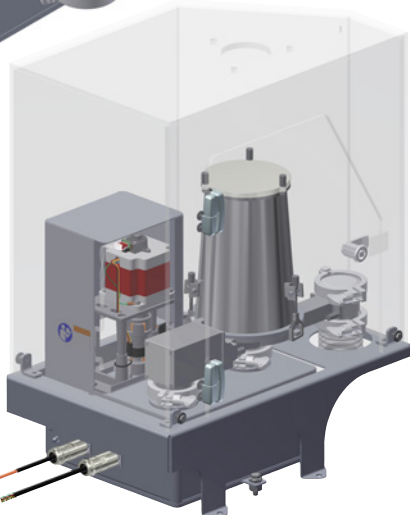
above: 16mm Microfeeder with 6 liter hopper and optional impactor
