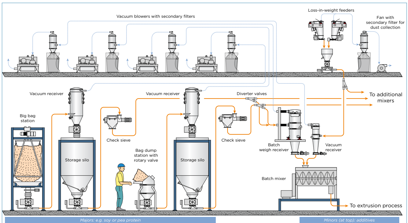
Figure 2 - Material handling from receipt to mixer
