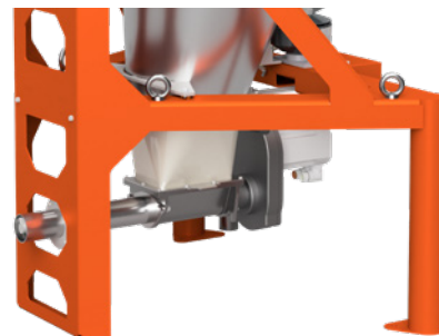
ProRate PLUS-M feeder with vertical outlet (above) and horizontal outlet (below).
